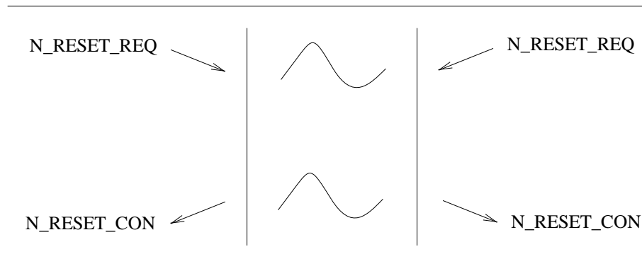
Figure 13. Sequence of Primitives: Simultaneous NS User Invoked Reset
