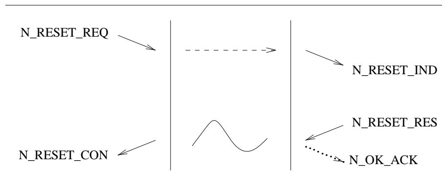
Figure 12. Sequence of Primitives: NS User Invoked Reset
