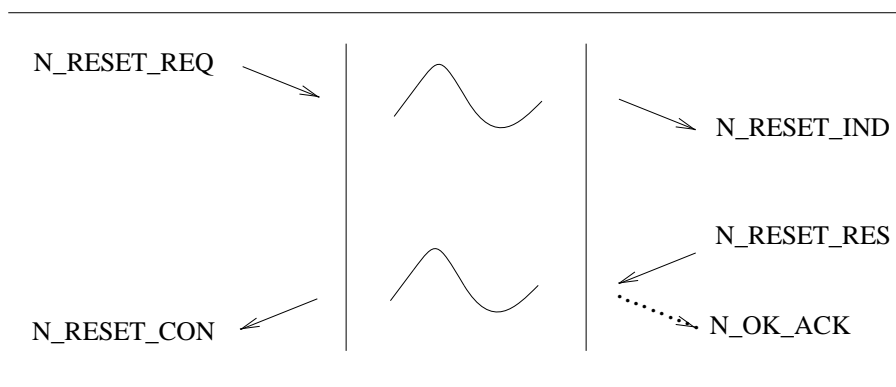
Figure 15. Sequence of Primitives: Simultaneous NS User & NS Provider Invoked Reset
