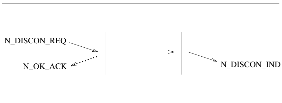
Figure 16. Sequence of Primitives: NS User Invoked Release
