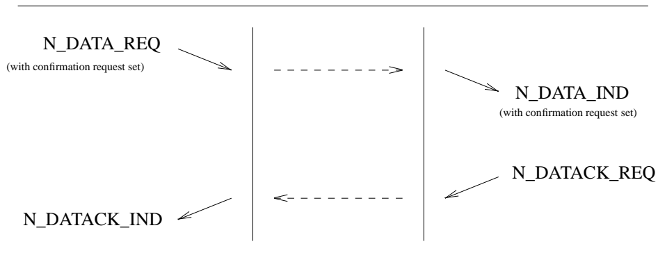
Figure 10. Sequence of Primitives: Successful Confirmation of Receipt
