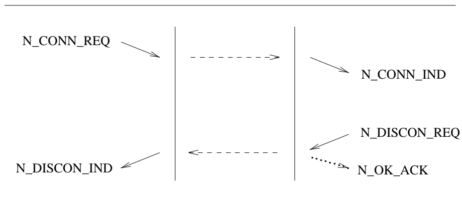
Figure 20. Sequence of Primitives: NS User Rejection of an NC Establishment Attempt
