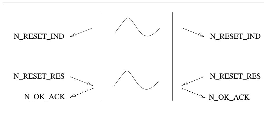
Figure 14. Sequence of Primitives: NS Provider Invoked Reset
