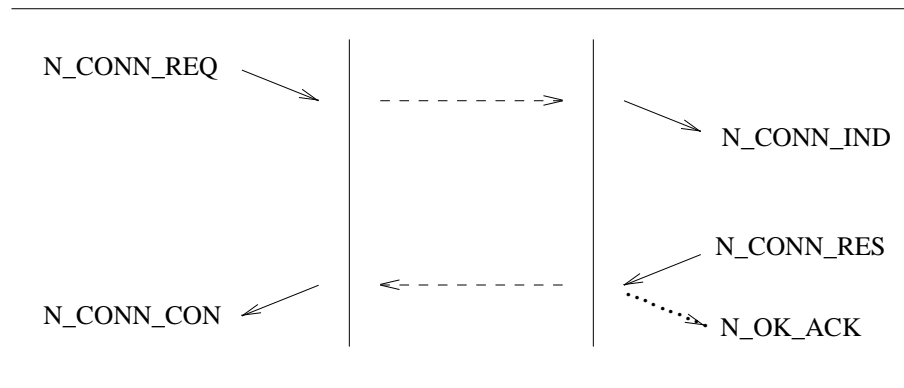
Figure 7. Sequence of Primitives: Successful NC Establishment
