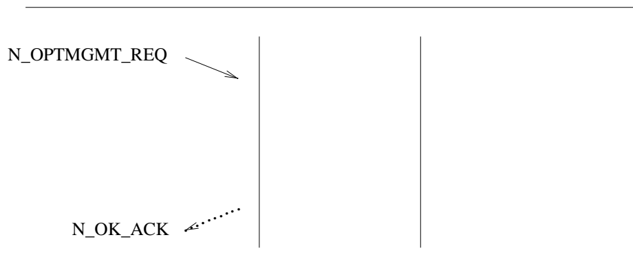
Figure 5. Sequence of Primitives: Options Management Service
