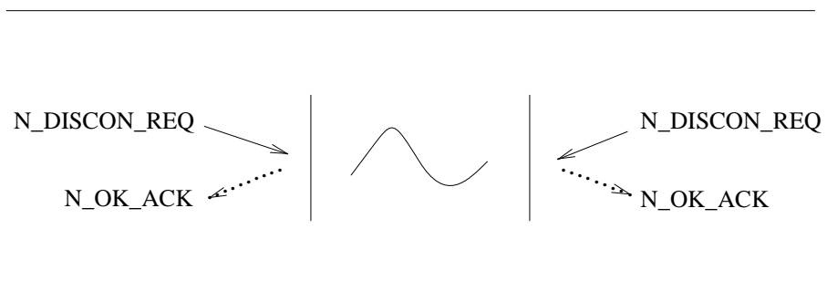
Figure 17. Sequence of Primitives: Simultaneous NS User Invoked Release
